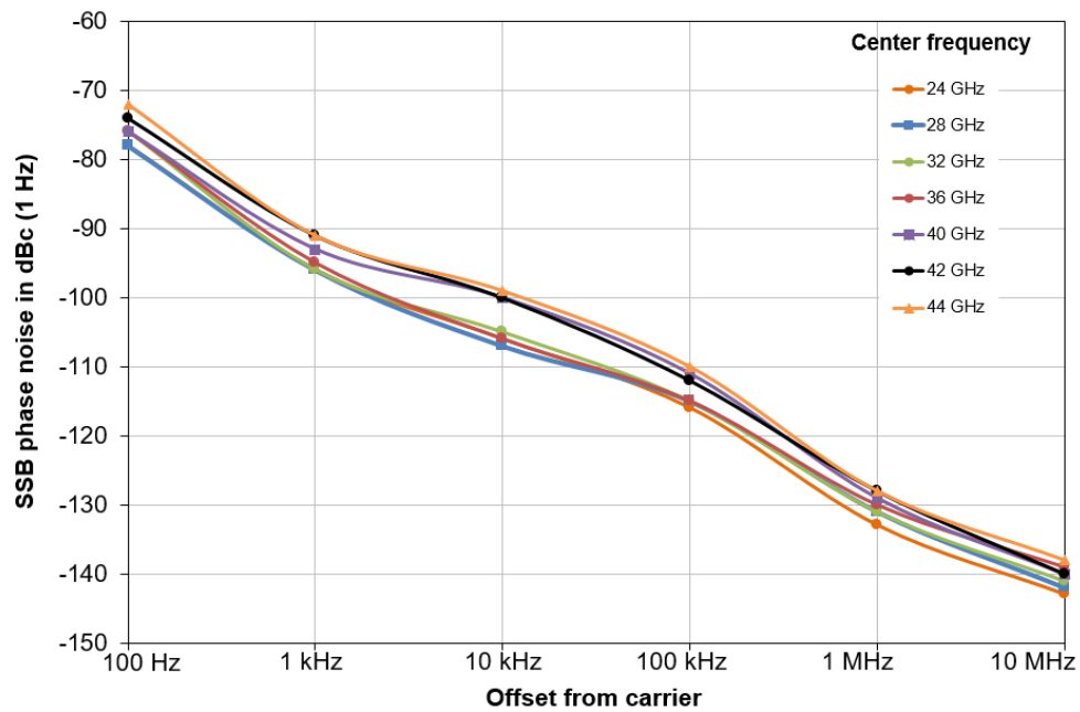
Typical single side band phase noise at different center frequencies in combination with an R&S®FSVA3000
