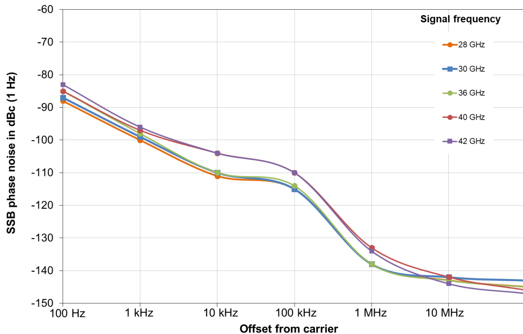
Typical single side band phase noise at different center frequencies in combination with an R&S®SMW200A
