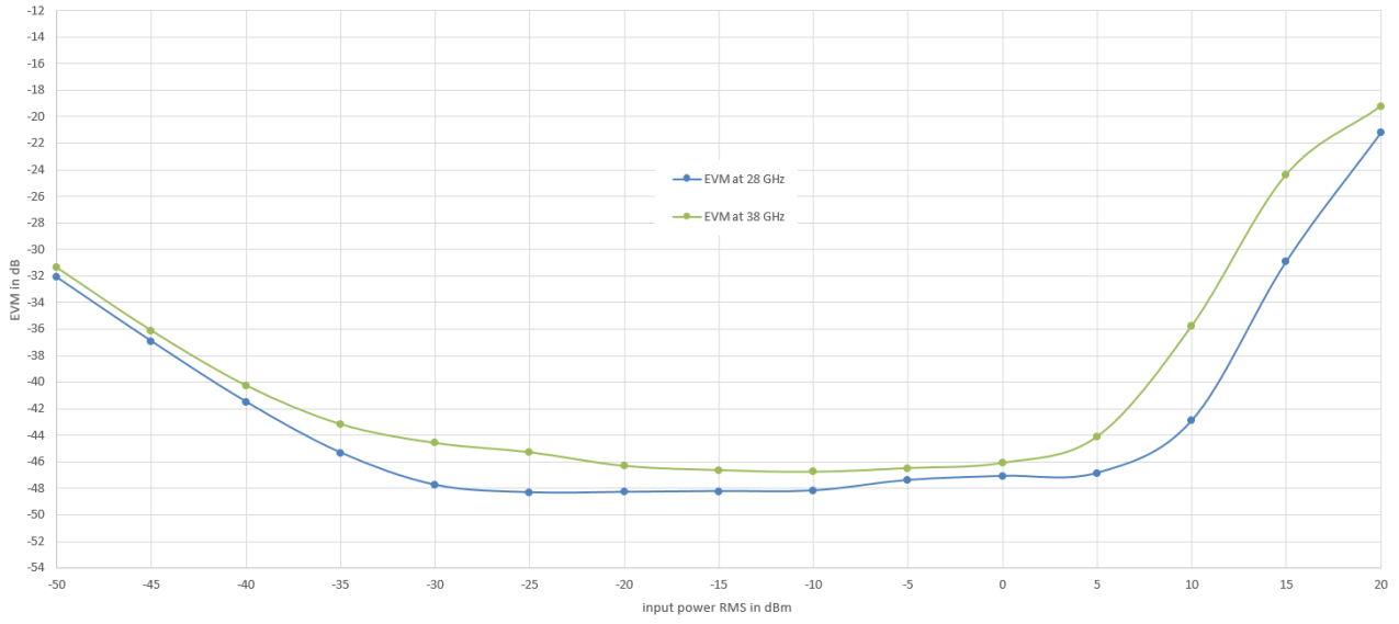
EVM values versus input power at different center frequencies in combination with an R&S®FSVA3000 (IF mode = low)
