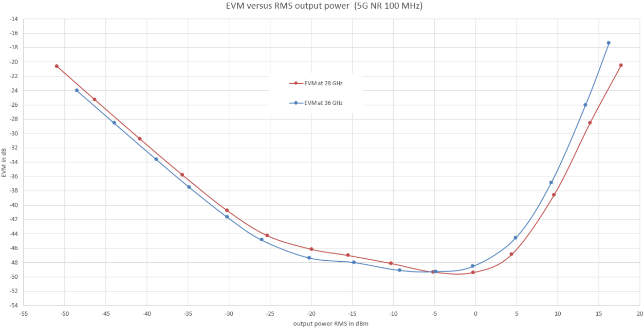
EVM values versus output power at different center frequencies in combination with an R&S®SMW200A (IF mode = low)
