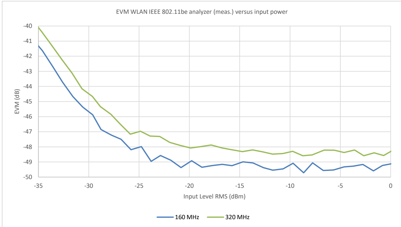
EVM WLAN IEEE 802.11be analyzer versus input power at 6985 MHz (meas.)
