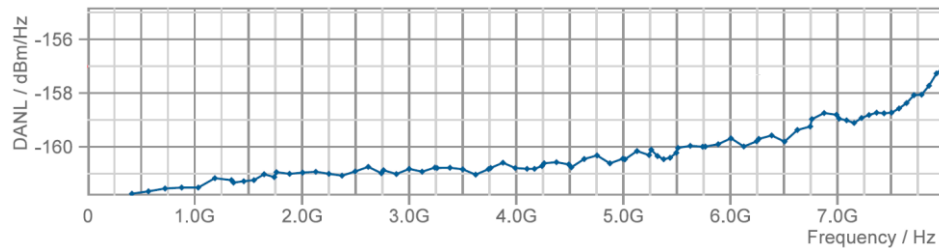
RX DANL measured values (meas.)
