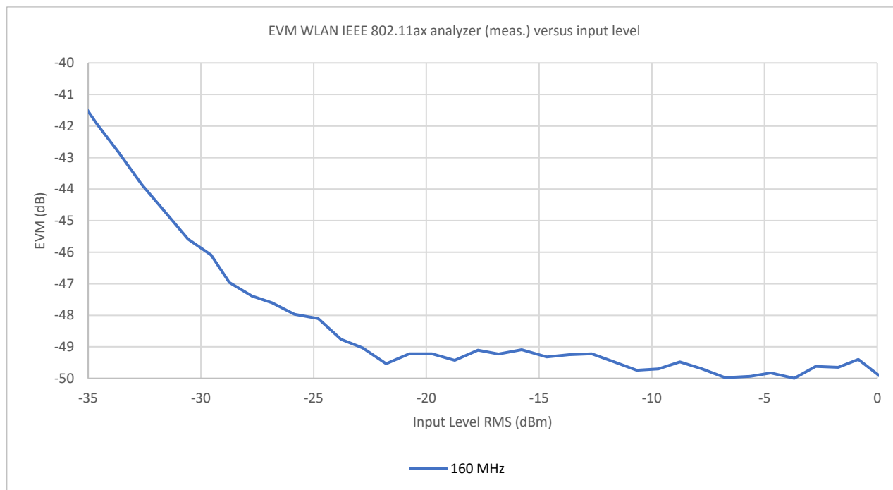
EVM WLAN IEEE 802.11ax analyzer versus input level at 6985 MHz (meas.)
