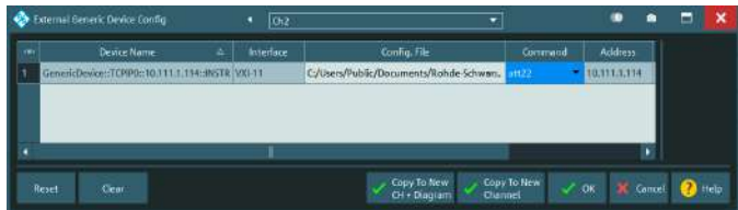
A JASON command list file is defined in the "External Generic Device Config" menu. A command or command sequence from the file can be selected for each channel.
