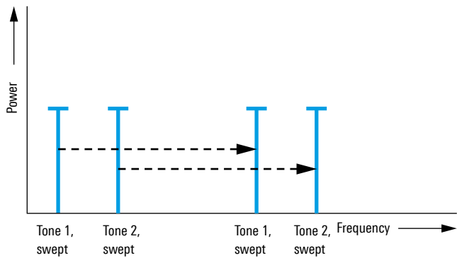
Frequency sweep with fixed carrier spacing
