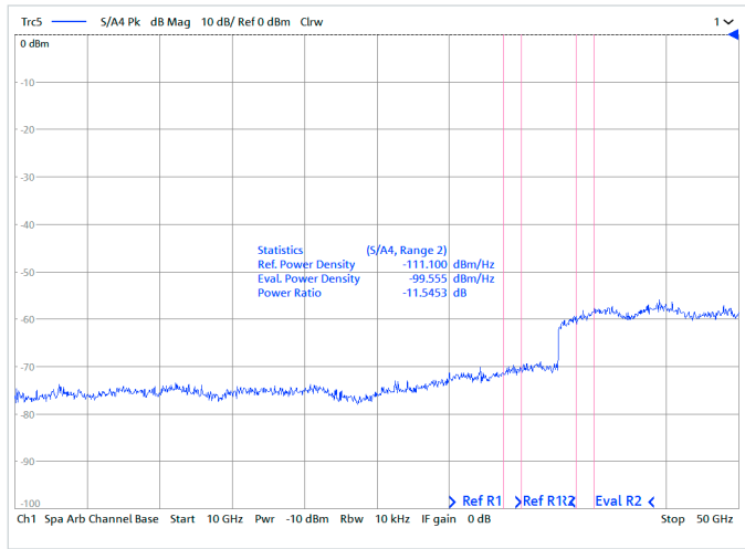
R&S®ZNA-K1 analysis functions: display of the ratio of power densities from different segments and the noise power marker function
