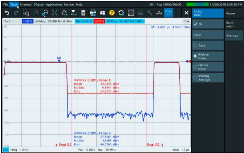
Pulse profile measurement: the wideband measurement mode enables single-shot pulse sweeps without averaging. Averaging (AVG) modes are also available to achieve either a very low trace noise or a very high dynamic range (i.e. a high pulse on/off ratio) based on vector averaging. Red trace: AVG mode "flatten noise". Blue trace: AVG mode "reduce noise".
