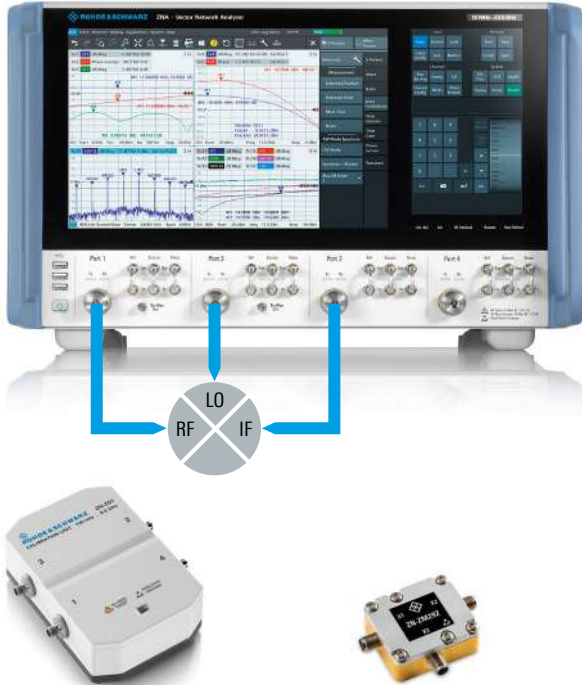
R&S®ZN-25x automatic calibration unit R&S®ZN-ZM292 calibration mixer
