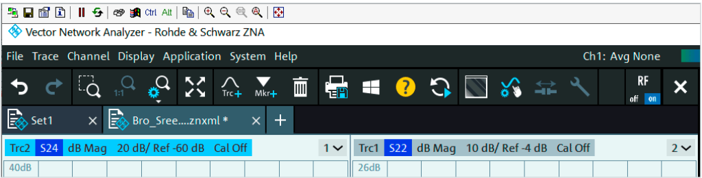
The TightVNC viewer allows full remote access and operation of an R&S®ZNA and adds valuable features such as file exchange and control command execution.
