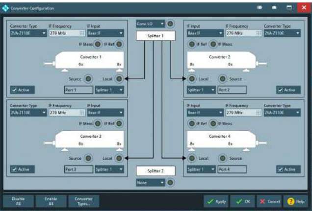
Software configuration
