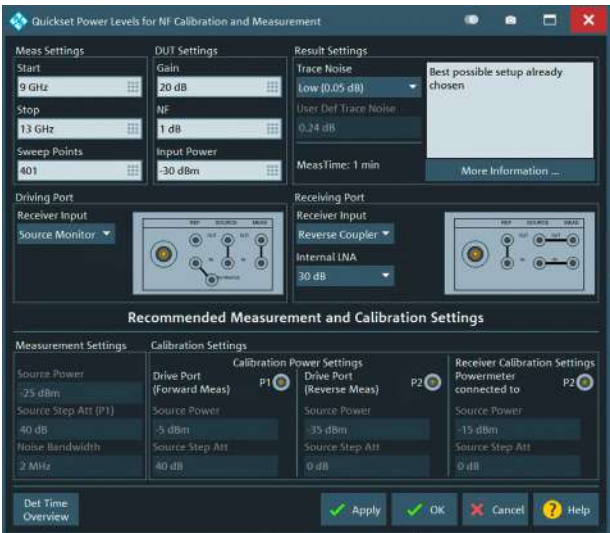
Quickset dialog for interactive and semi-automatic configuration of optimal test parameters and R&S®ZNA hardware
