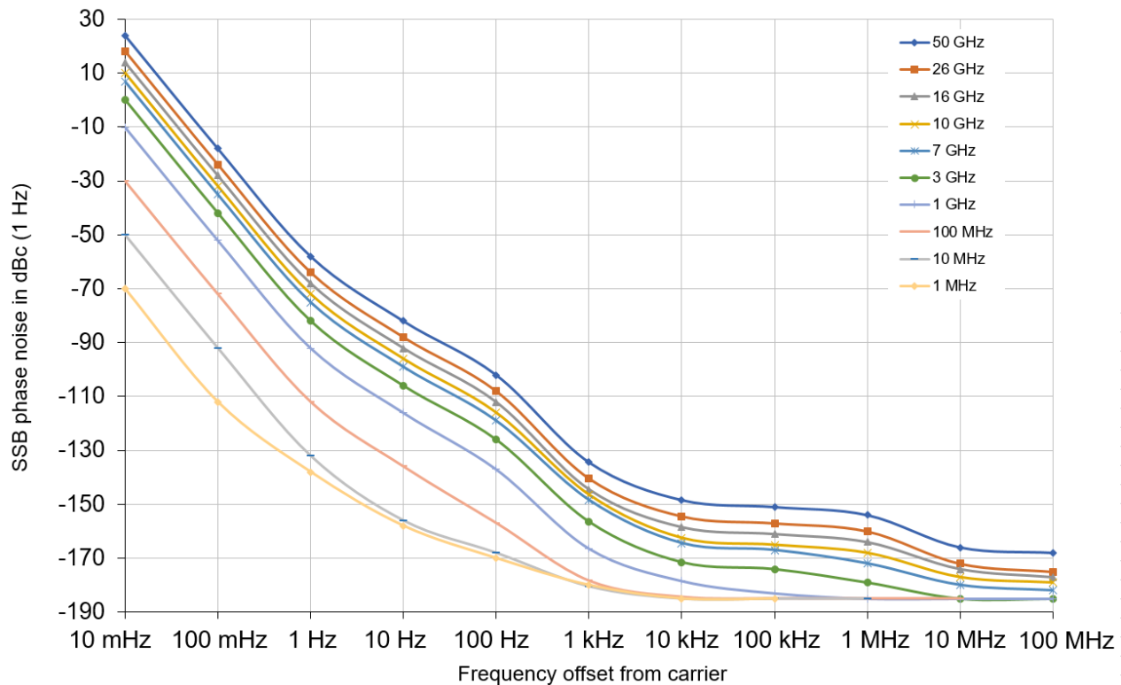
Typical phase noise at different center frequencies with R&S®FSWP-B61 option (start offset = 10 mHz)
