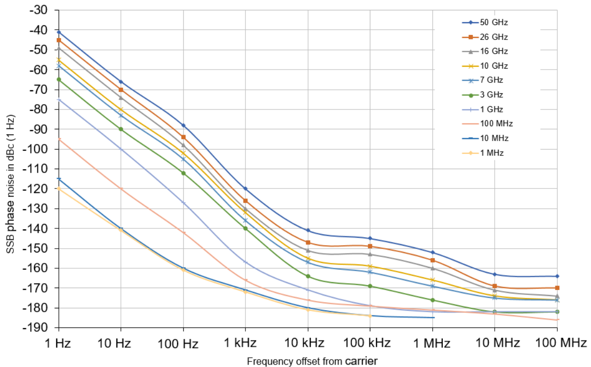
Typical phase noise at different center frequencies with R&S®FSWP-B60 option (start offset = 1 Hz)
