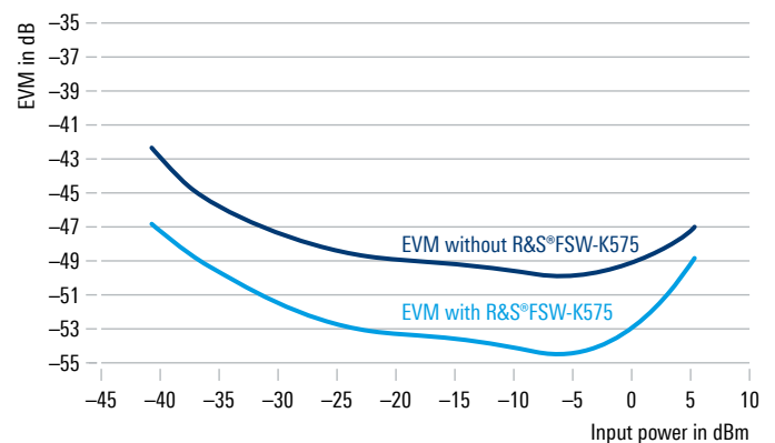
Residual EVM over signal power for a 320 MHz Wi-Fi 802.11be signal at 6.905 GHz (modulation order 4096 QAM)
