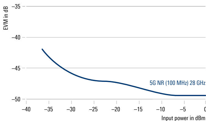
Residual EVM over signal power for a 100 MHz wide 5G NR uplink signal at 28 GHz
